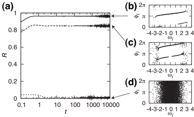
FIG. 2. (a) Time evolution of the order parameter R from three different initial conditions in the mean field model with N = 10,000 and K = 3 . (b,c,d) \omega_i - \phi_i relationship for different initial conditions at t = 10,000 .
