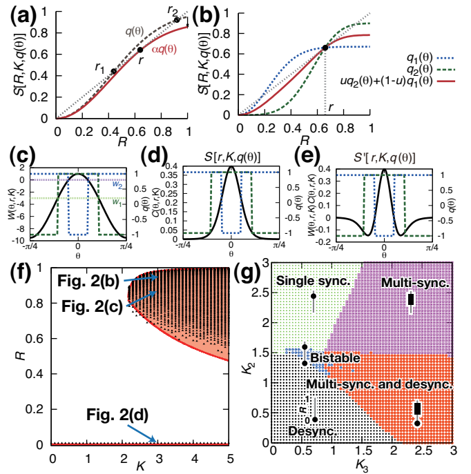
FIG. 3. (color online). (a) For some q(\theta) , the self-consistent equation R = S[R, K, q(\theta)] have two solutions, r_1 < r_2 (brown line). Setting \alpha appropriately makes R = S[R, K, \alpha q(\theta)] have only one solution R = r < r_2 (red line). Note that S'[r, K, \alpha q(\theta)] = 1 . (b) If we have S[r, K, q_1(\theta)] = r and S'[r, K, q_1(\theta)] = s_1 \leq 1 (blue line) and S[r, K, q_2(\theta)] = r and S'[r, K, q_2(\theta)] = s_2 \geq 1 (green line), we can obtain q(\theta) with which S[r, K, q(\theta)] = r and S'[r, K, q(\theta)] = 1 hold (red line). (c,d,e) q_2(\theta) which maximizes S'[r, K, q(\theta)] (e) under the constraint S[r, K, q(\theta)] = r (d) is given by q_2(\theta) = 2\Theta[W(\theta, r, K) - w_2] - 1 (green line) where w_2 is set to satisfy S[r, K, q_2(\theta)] = r (c). Under the same constraint, S'[r, K, q_1(\theta)] is minimized by q_1(\theta) = 2\Theta[w_1 - W(\theta, r, K)] - 1 (blue line) where S[r, K, q_1(\theta)] = r . (f) Attainable region of the order parameter R (orange region). Note that the incoherent state R = 0 is stable for any K (red line). (g) Phase diagram of the system of phase oscillators when the strength of two-body and three-body interactions are changed. The symbol in each region is a schematic representation of the attainable values of the order parameter R . Gray lines represent the range of R from 0 to 1. The attainable values and ranges of R are indicated by black circles and boxes, respectively.
