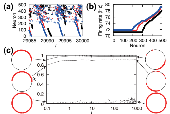
FIG. 1. (color online). Two examples of multistability arising from three-body interaction. (a) Raster plot of the spikes in a network of the Hodgkin-Huxley neurons with short-term heterosynaptic plasticity ( N = 500 ). Black, red, and blue dots represent the firings in the networks starting from different initial conditions. Neurons are sorted in ascending order of the firing rate. Firing rate of each neuron is shown in (b). (c) Time evolution of the order parameter R for three different initial conditions in the phase-oscillator systems with non-uniform random coupling ( N = 500 ). Phase distributions of oscillators at t = 0 and t = 1,000 are shown on the left and right, respectively. These two examples demonstrate that the same system can show different degrees of synchrony depending on the initial conditions.
